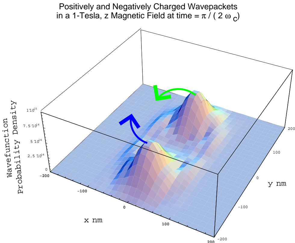
Figure 4: The wave packet used in figures 5 through 7.
