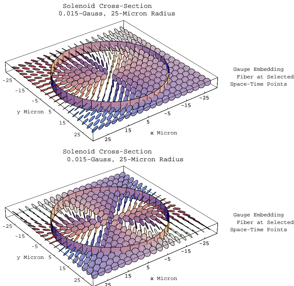
Figure 3: The cross-section of a solenoid of radius R = 25 \mu\text{m} , with a magnetic field strength of B_o = 0.015 \text{ Gauss} . The diagram shows eqs. (5.9) and (5.10) for two vacuum topologies, n = 1 in the top figure and n = 2 in the bottom figure. The cylinder represents the solenoid boundary.
