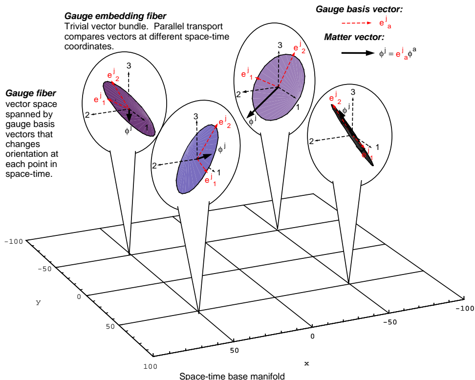
Figure 1: An \mathbb{R}^2 -vector bundle embedded in a trivial \mathbb{R}^3 -vector bundle. The choice of gauge determines the dotted-red basis vectors of the gauge fiber. The thick black vectors of varying length represent a real scalar matter field, which can be interpreted as a wavefunction.
