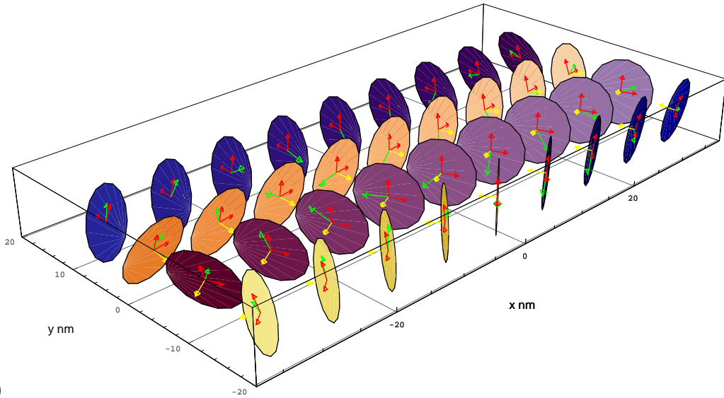
Figure 6: The first method to incorporate two matter fields with different charges. These two figures show two independent gauge fibers over the same space-time. Part (a) shows a magnetic field with positive curvature, and part (b) shows a magnetic field with negative curvature. Without an external constraint, nothing restricts the curvature of the two fibers to have any relation to each other.
