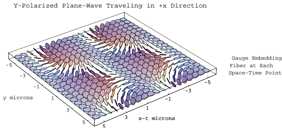
Figure 2: \hat{y} -polarized plane wave (5.8) propagating in the positive \hat{x} direction. The figure corresponds to radiation with \lambda = 10.6 \mu\text{m} and intensity of \approx 6.4 \text{ Watts/mm}^2 .
